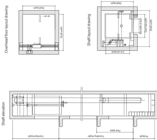
Machine roomless passenger specifications
