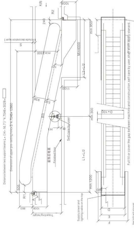
12° Moving walk construction layout drawing
