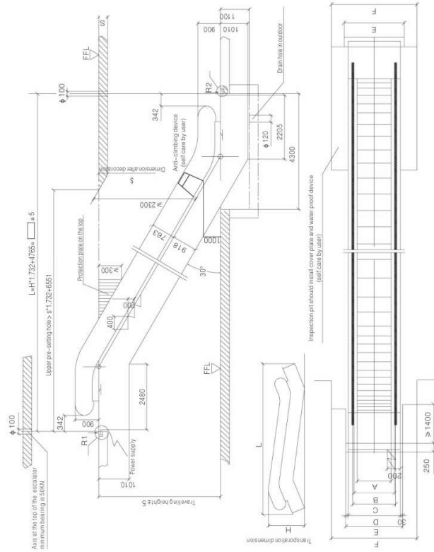
30° Escalator construction layout drawing
