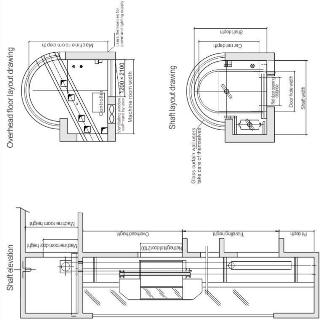
Semicircle machine room / Machine roomless elevator specifications
