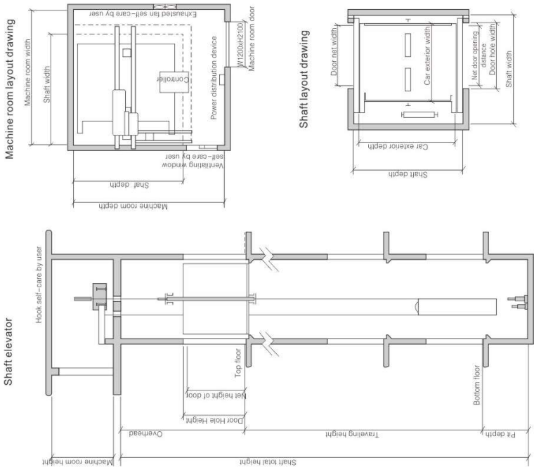
Freight elevator specifications
