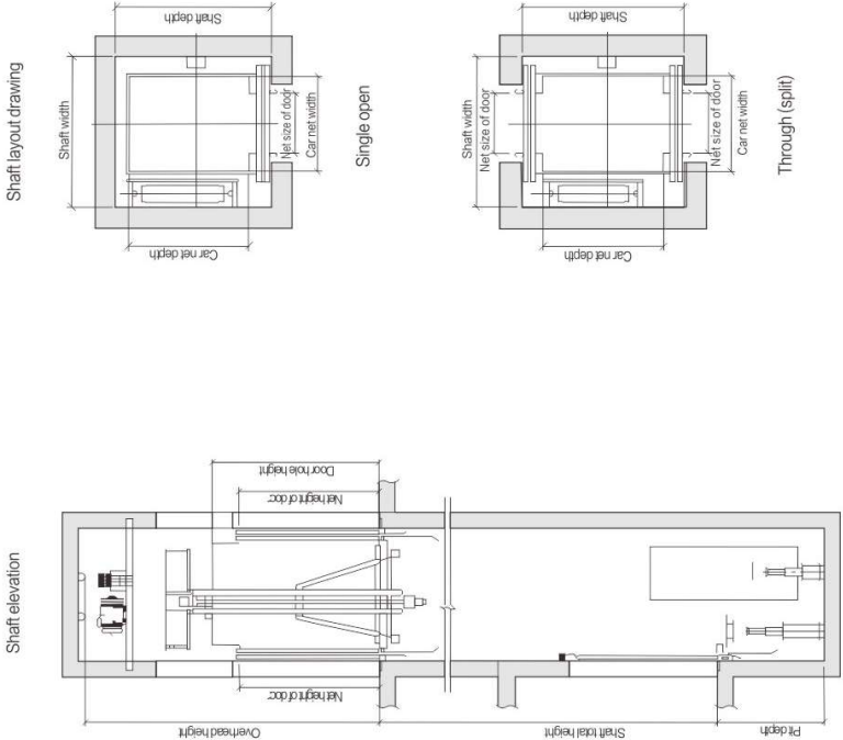
Steel structure elevator specifications
