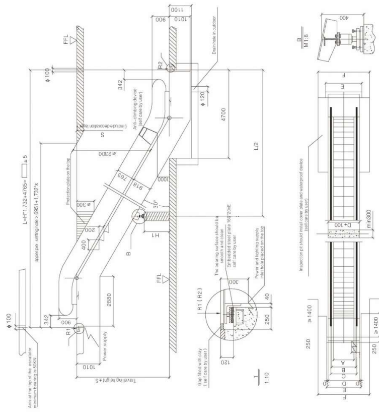
Large height escalator construction layout drawing
