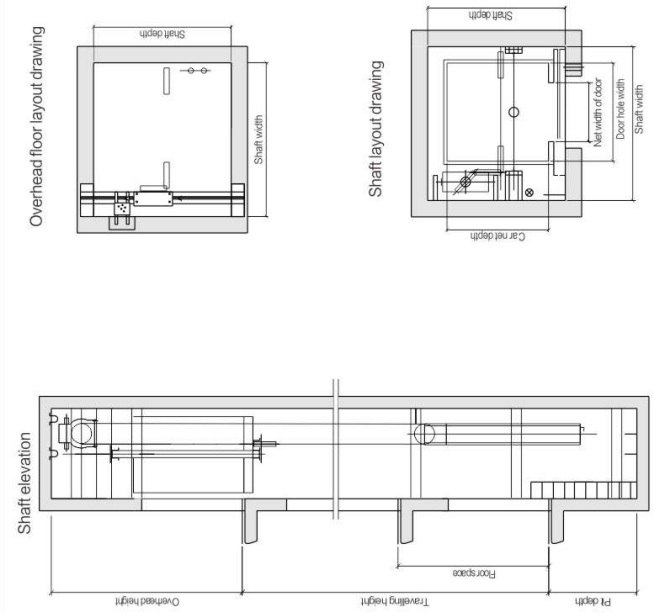
Square machine room / Machine roomless elevator specifications
